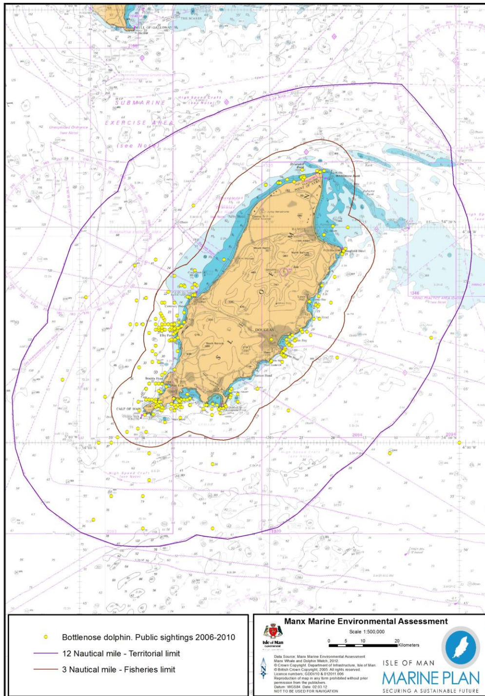
Figure 12. Draft Map – Opportunistic sightings of Bottlenose dolphin from public reports to MWDW (2006-2010).
