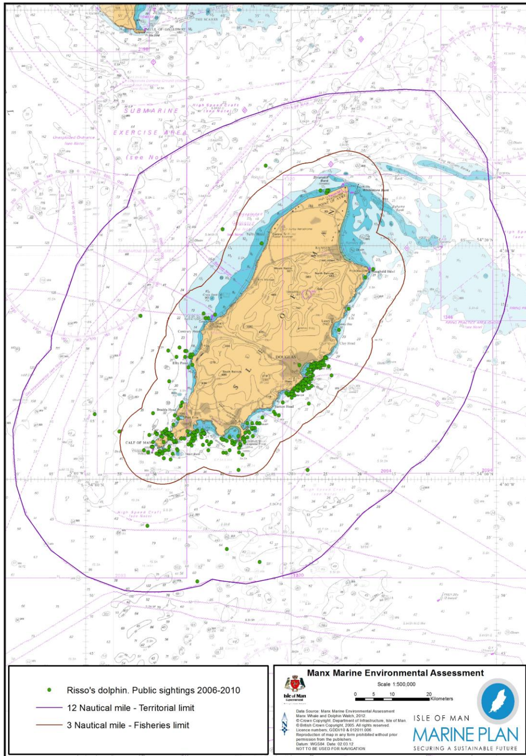
Figure 7. Draft Map – Opportunistic sightings of Risso’s dolphin from public reports to MWDW (2006-2010).
