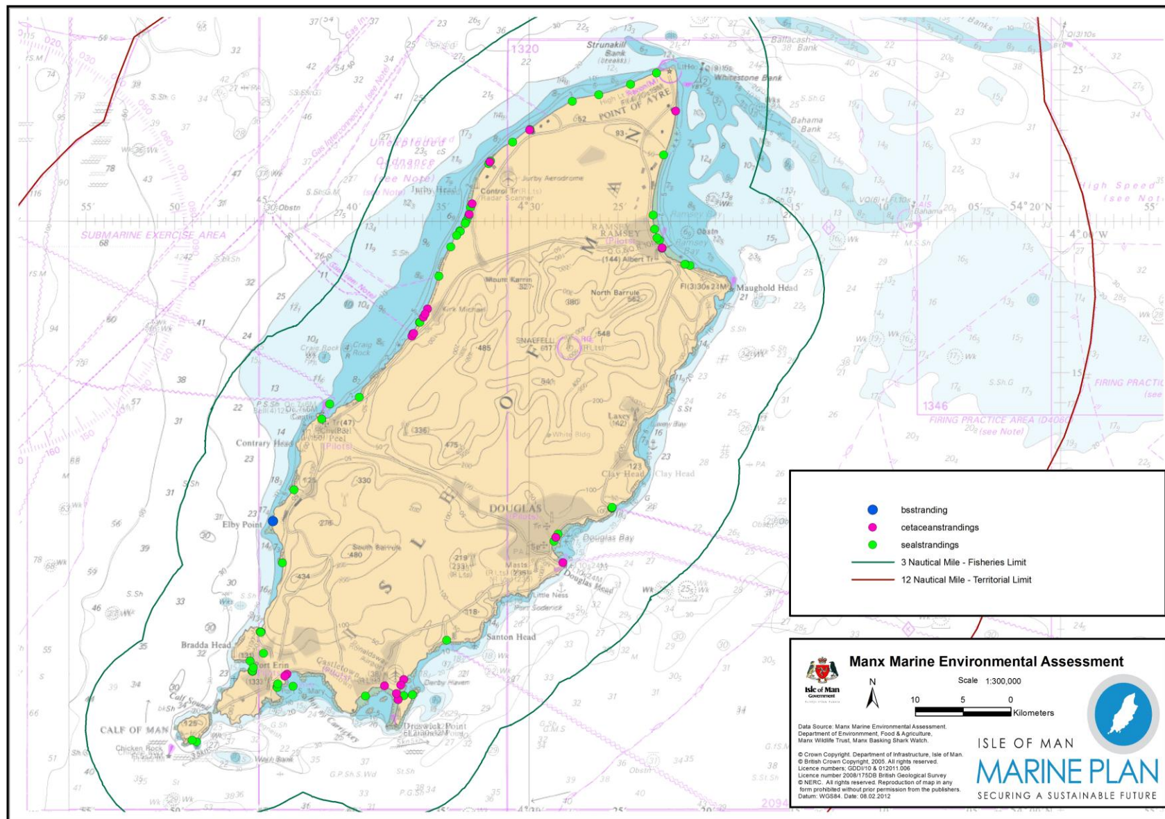
Figure 3. Draft Map - The distribution of stranded cetaceans recorded by DEFA between 2008 and 2010.
