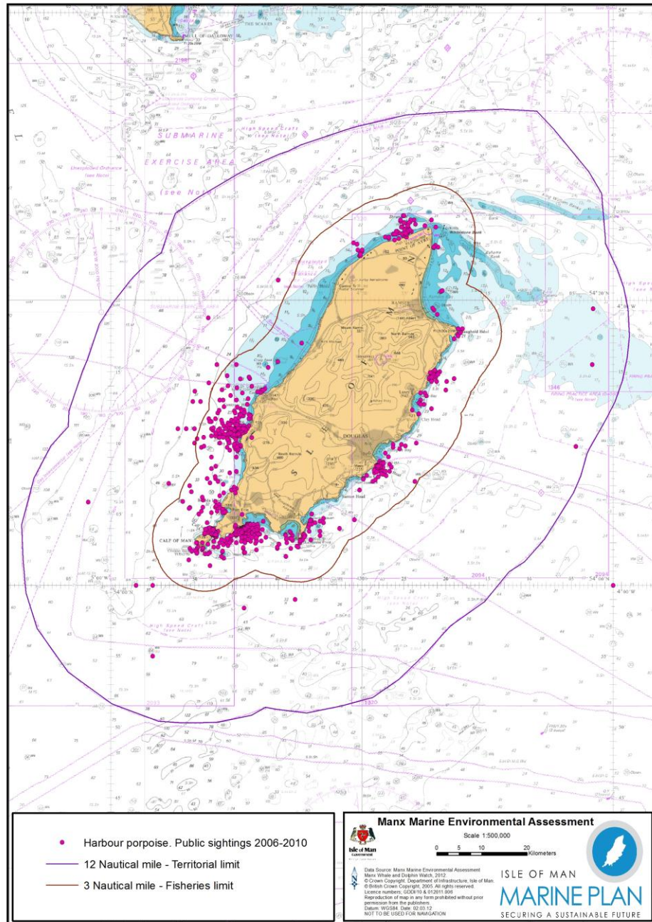
Figure 6. Draft Map - Opportunistic sightings of harbour porpoise from public reports to MWDW (2006-2010).
