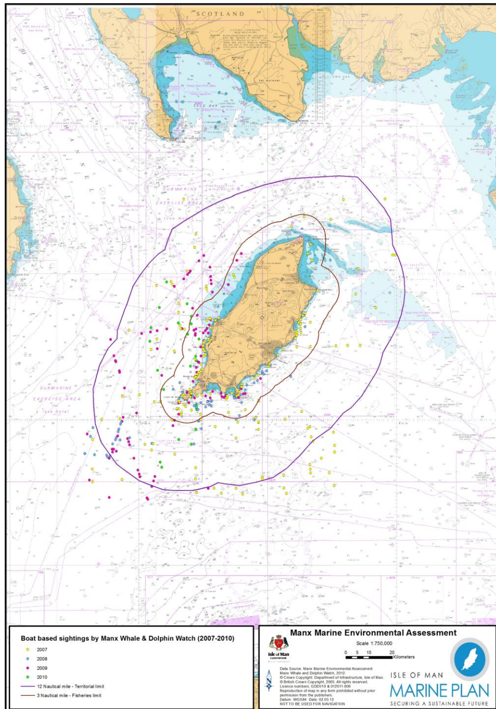
Figure 2. Draft Map - Locations where cetaceans were observed during effort based boat surveys (2007-2010).
