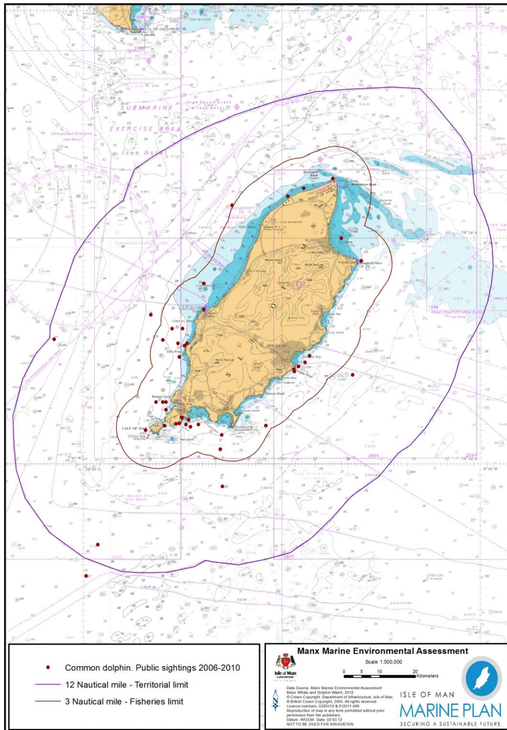
Figure 14. Draft Map – Opportunistic sightings of Common dolphin from public reports to MWDW (2006-2010).
