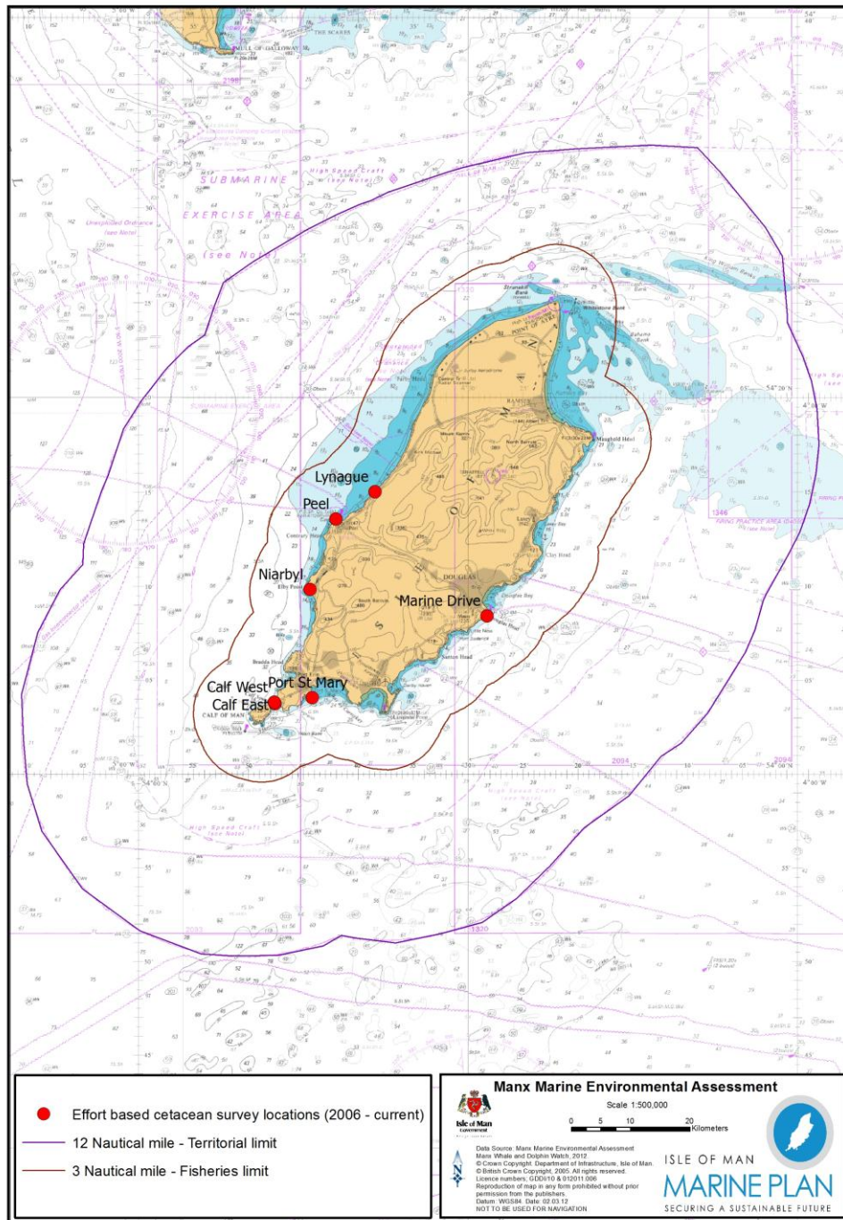
Figure. 1. Draft Map - MWDW Effort based survey locations, (2006 – current).
