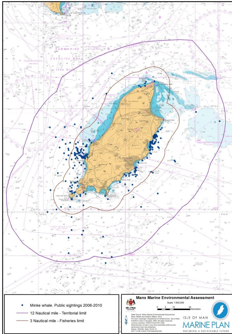
Figure 10. Draft Map – Opportunistic sightings of Minke whale from public reports to MWDW (2006-2010).
