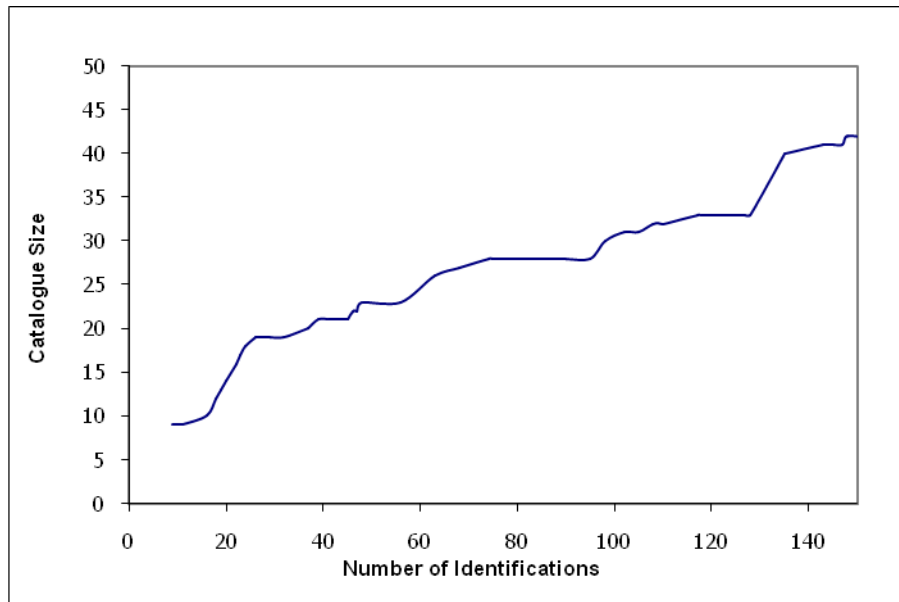
Discovery curve for Risso's Dolphin catalogue
